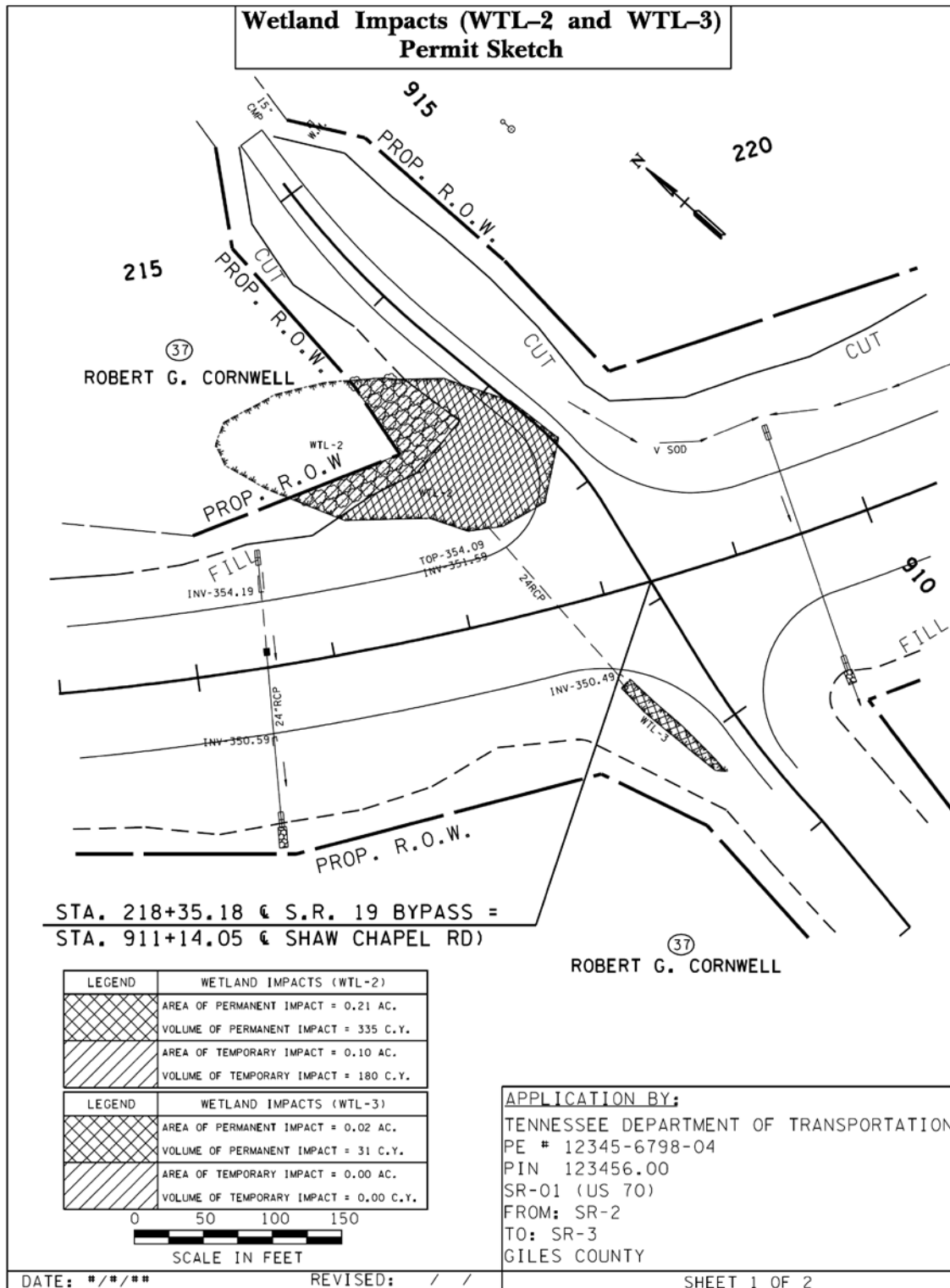
Figure 3-14 Example Permit Sketches for Wetland Impacts
