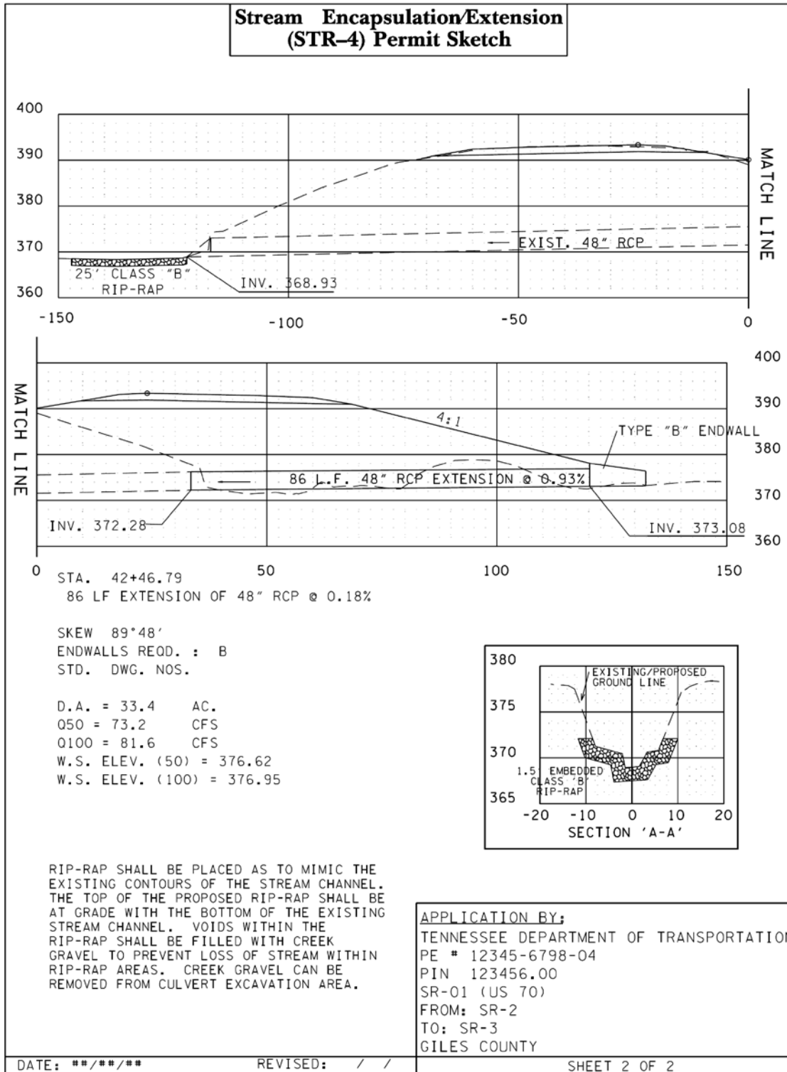
Figure 3-13 (Continued) Example Permit Sketch for Stream Encapsulation/Structure Extension
