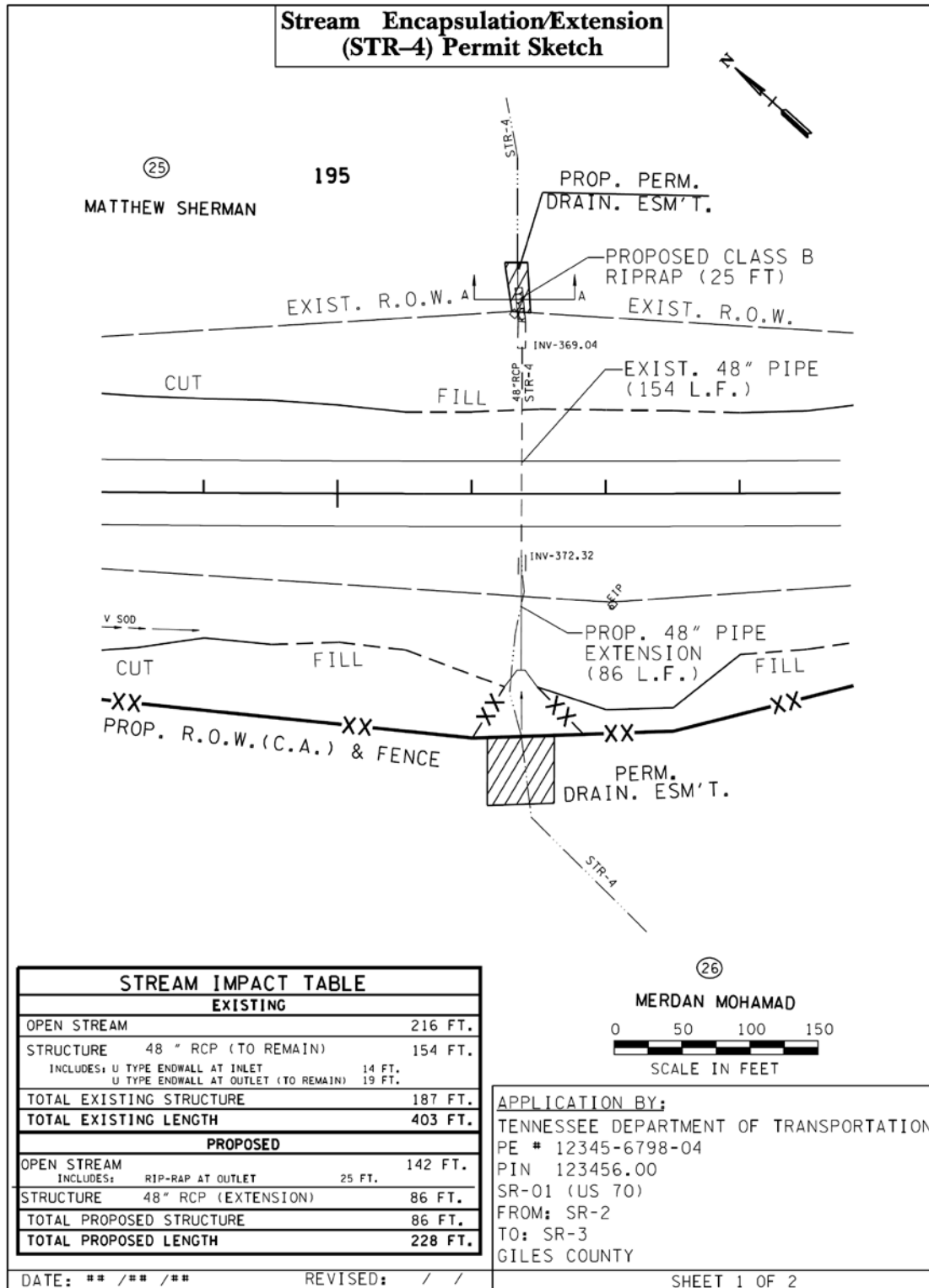
Figure 3-13 Example Permit Sketch for Stream Encapsulation/Structure Extension
