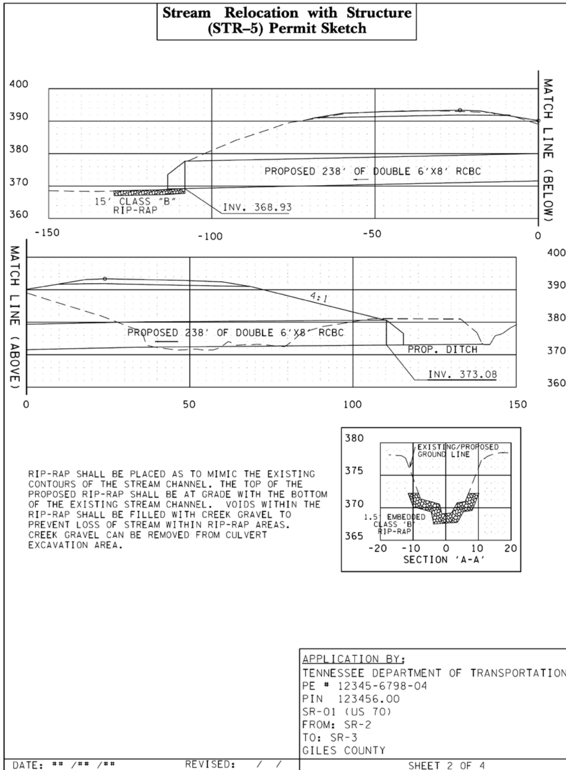
Figure 3-12 (continued) Example Permit Sketches for Stream Relocation with Structure
