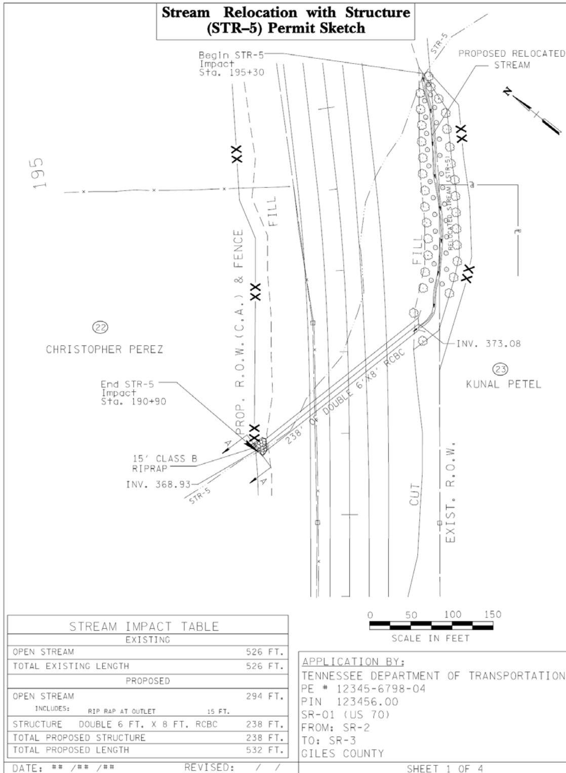
Figure 3-12 Example Permit Sketches for Stream Relocation with Structure
