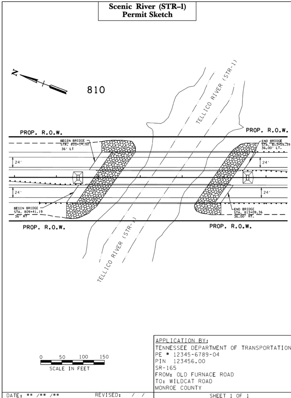
Figure 3-15 Example Permit Sketch for Scenic River Impacts
